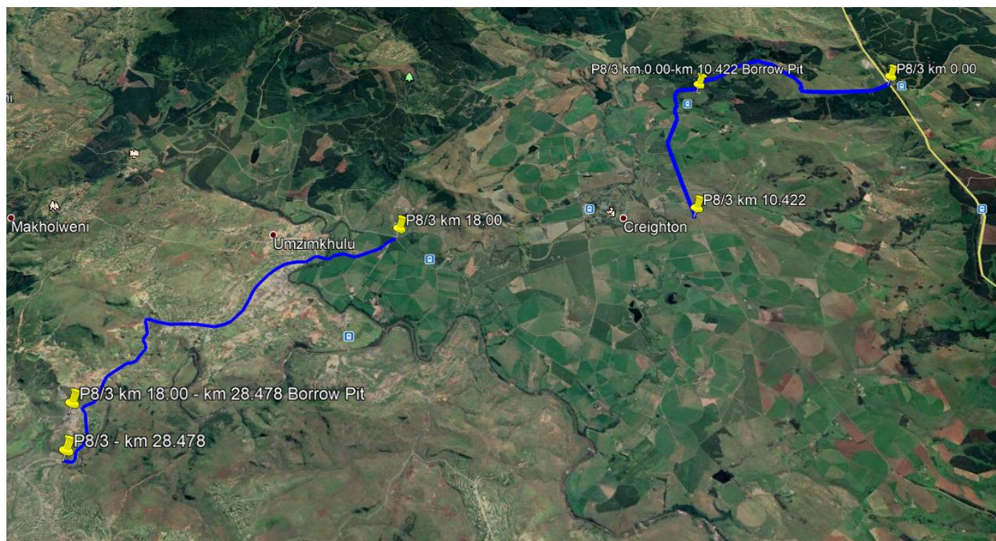
Figure C4.1 – Locality Plan of Main Road P8/3
